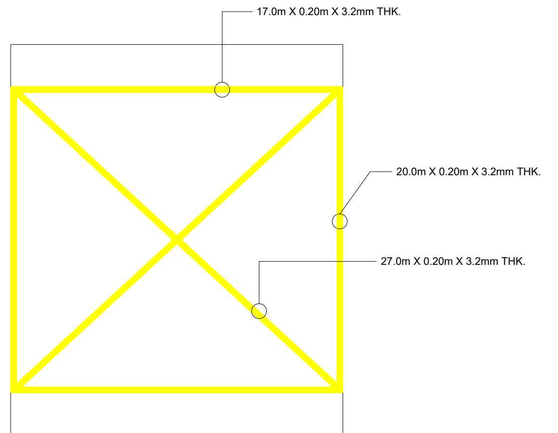
INTERSECTION ROAD MARKINGS - 19 UNITS
