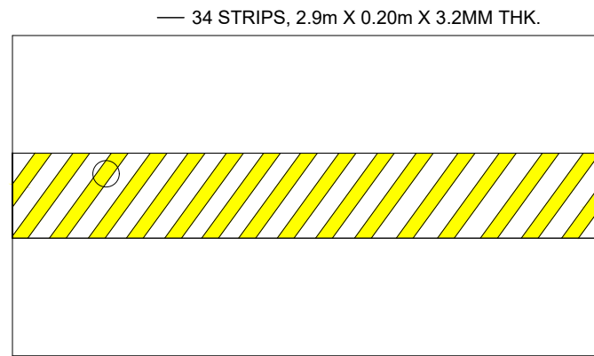
ROAD HUMPS - 24 UNITS (YELLOW THERMOPLASTIC PAINT)
