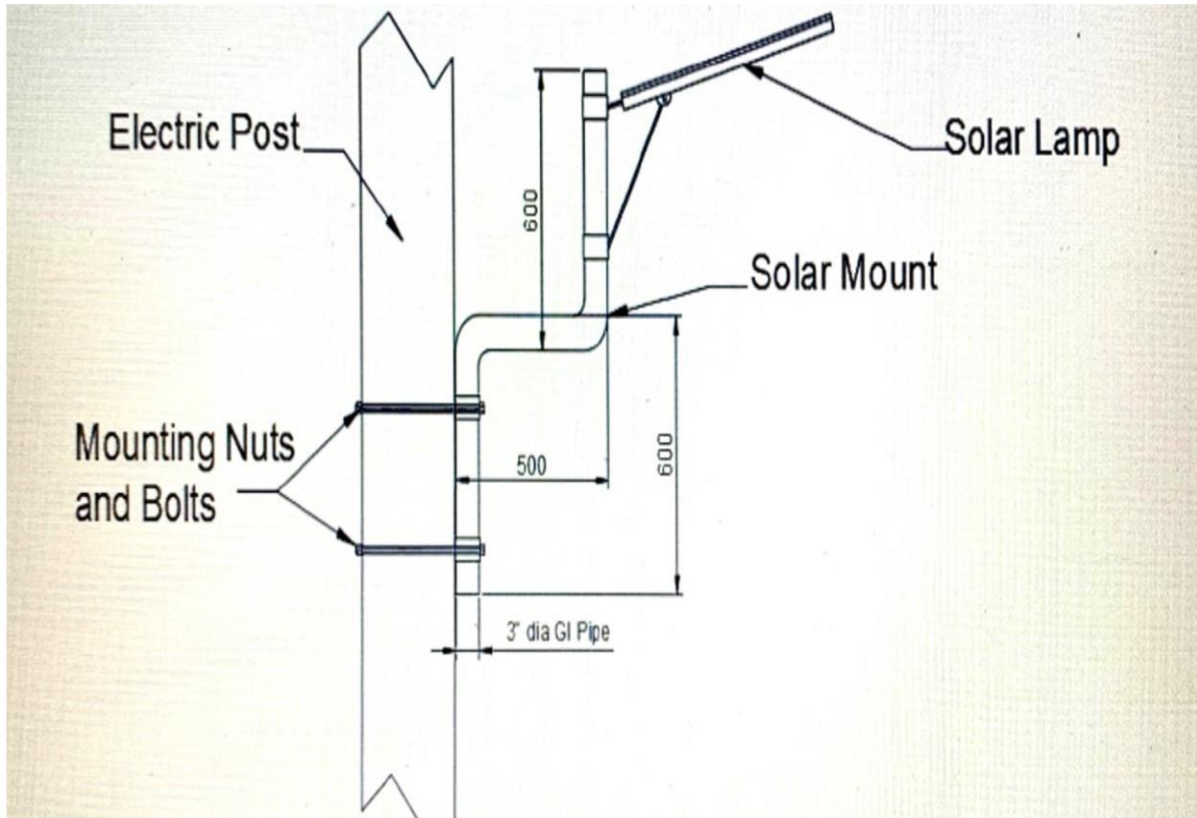
Solar Lights with Bracket for Electrical Posts
