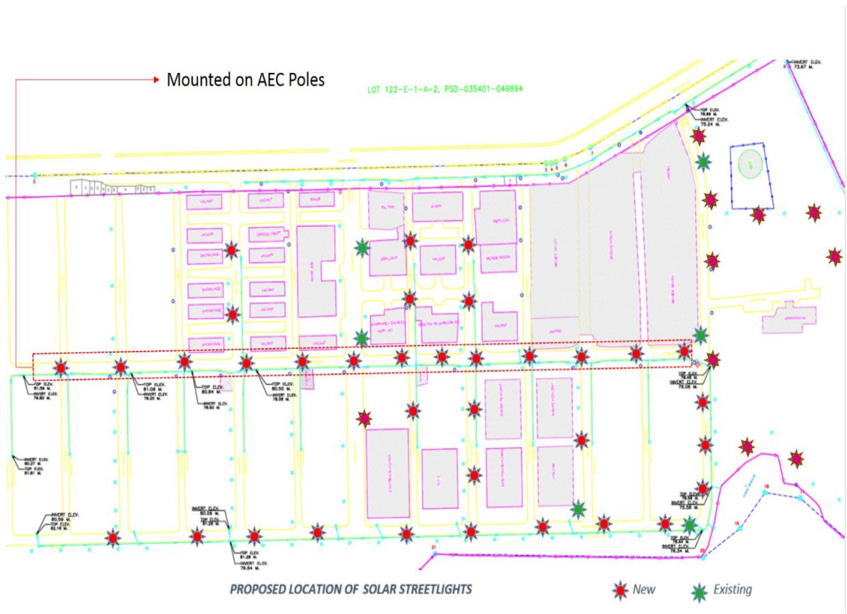
Solar Lights with Bracket for Electrical Posts
