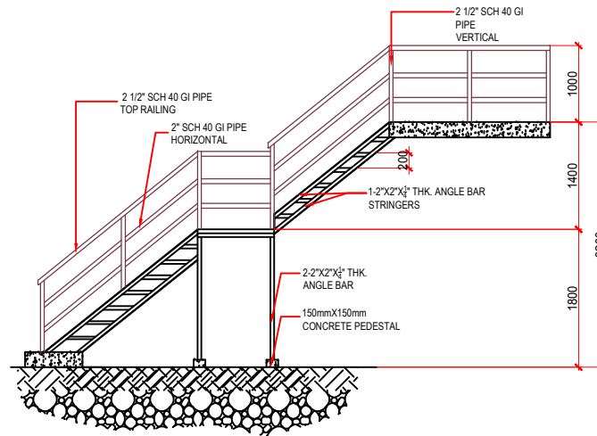
SECTION A
