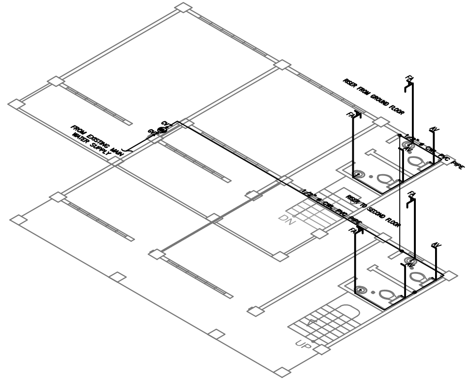
2 P-03 ISOMETRIC WATER LINE
