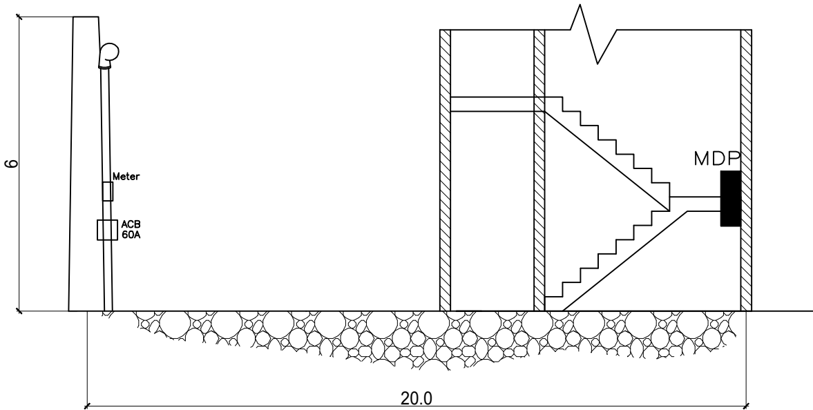
1 E-04 TRAINING CENTER SERVICE ENTRANCE
