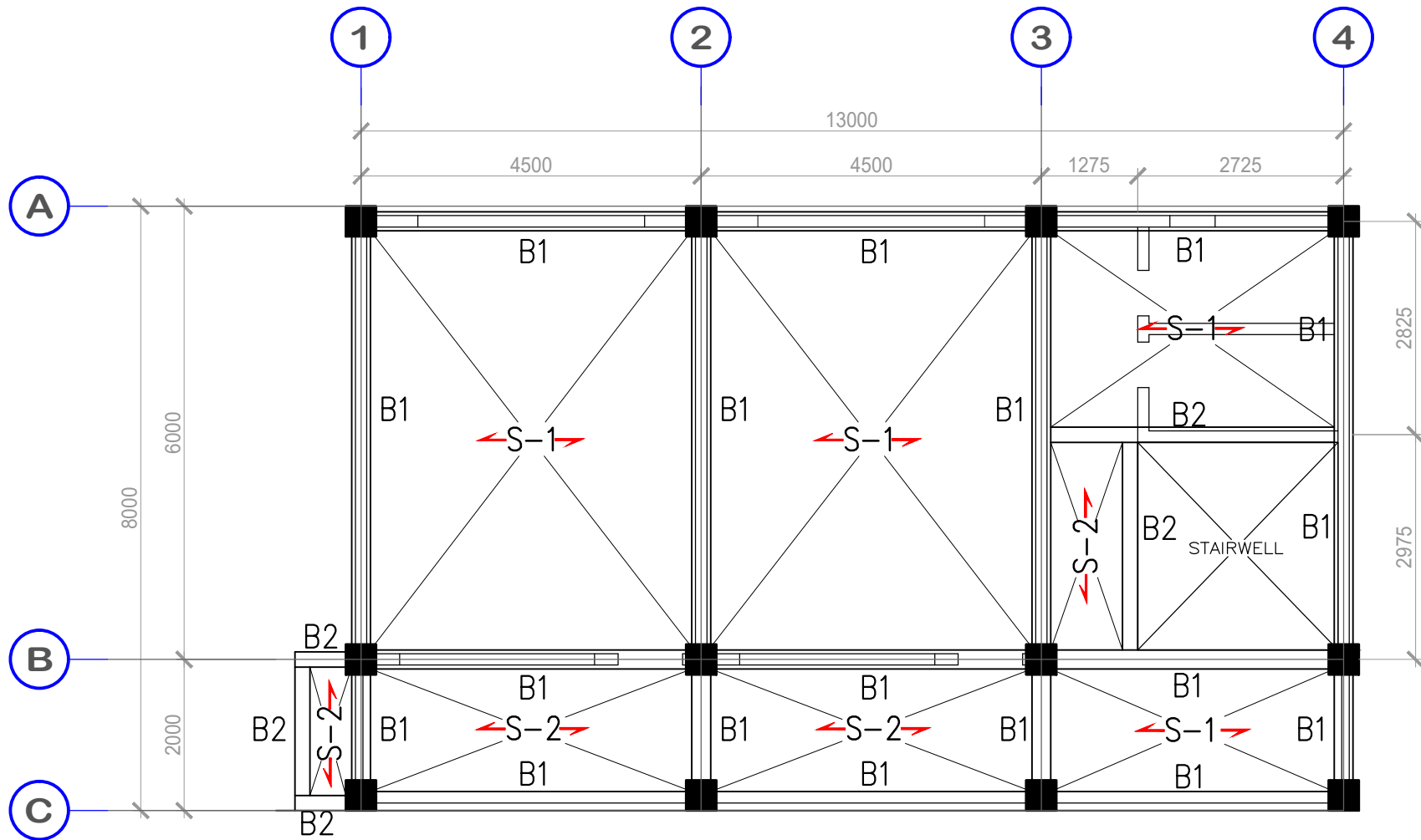
1 S-02 SECOND FLOOR FRAMING PLAN
