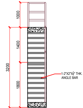
SECTION B
