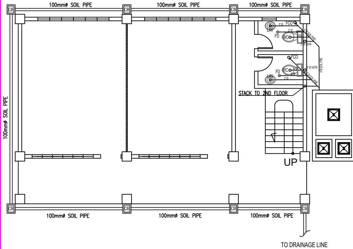
1 P-01 GROUND FLOOR SEWER LINE LAYOUT
