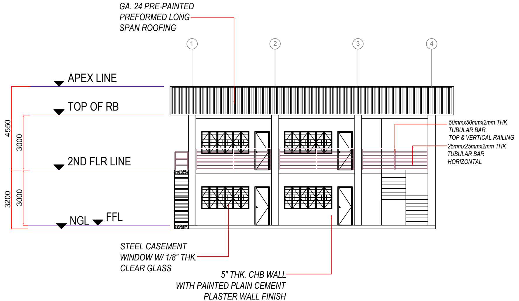
TRAINING CENTER FRONT ELEVATION
