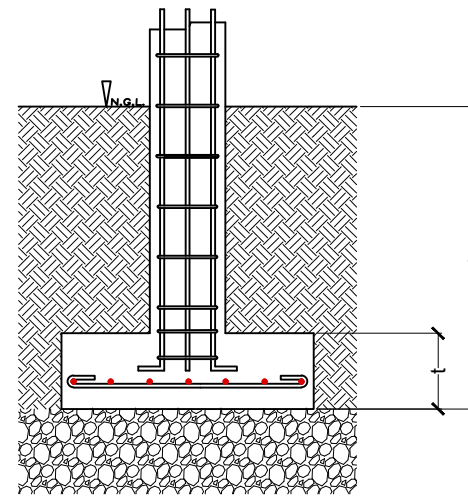
SECTION
