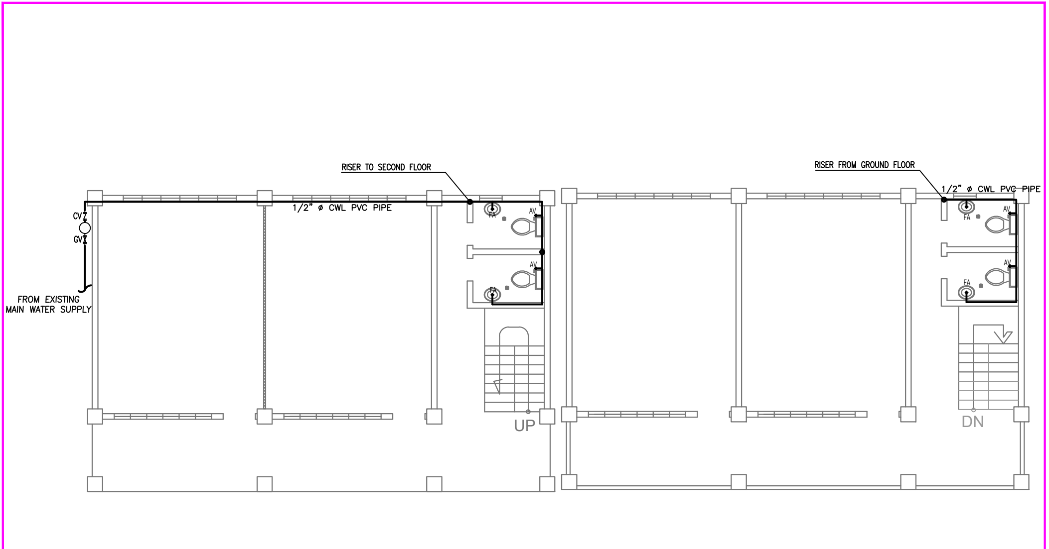
1 P-02 GROUND FLOOR WATER LINE LAYOUT
