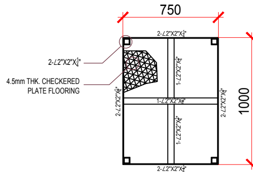
LANDING DETAILS
