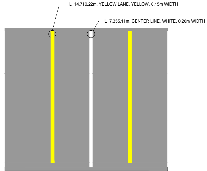
CENTER LINE AND YELLOW LANE
