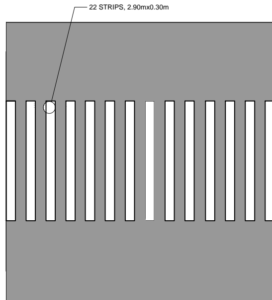
ZEBRA TYPE PEDESTRIAN LANE(24 Units)
