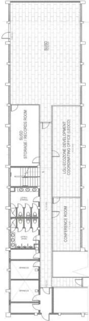
BUILDING 4B, GROUND FLOOR FLOOR FINISH PLAN 1:1000
