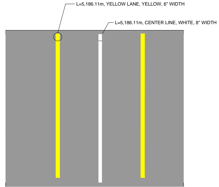
CENTER LINE AND YELLOW LANE
