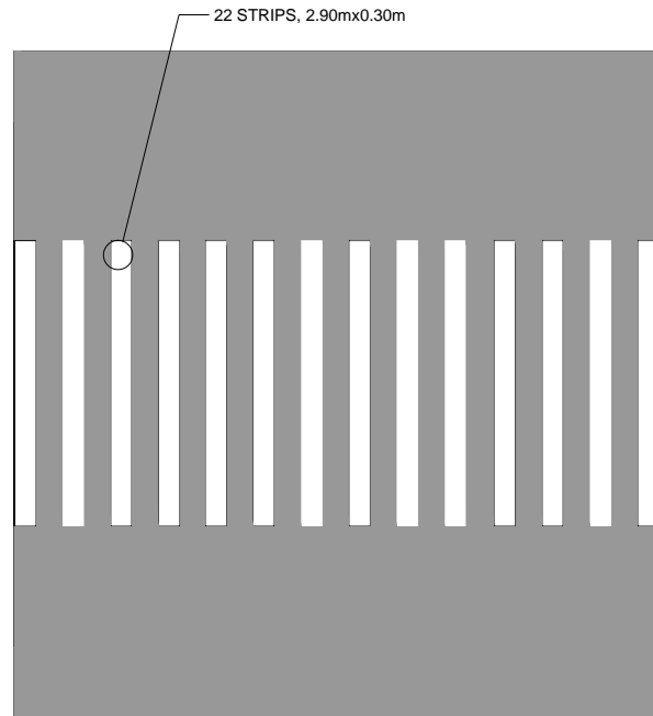
ZEBRA TYPE PEDESTRIAN LANE(5 Units)
