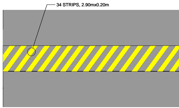
ROAD HUMPS (16 Units)
