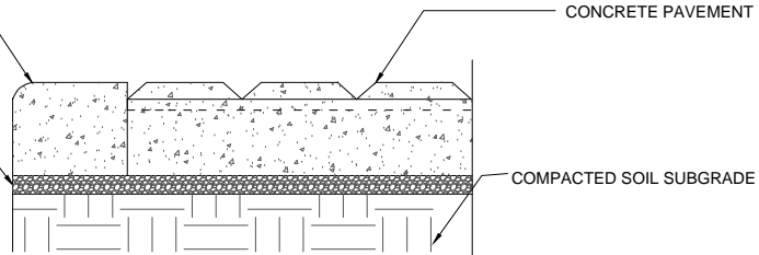
CONCRETE CURB SECTION DETAIL
