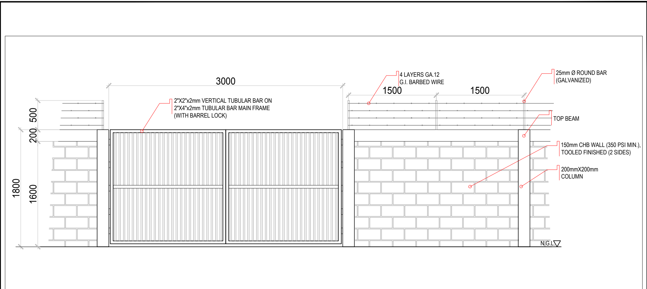
1 A-02 FENCE 1 TYPICAL ELEVATION 1:50M
