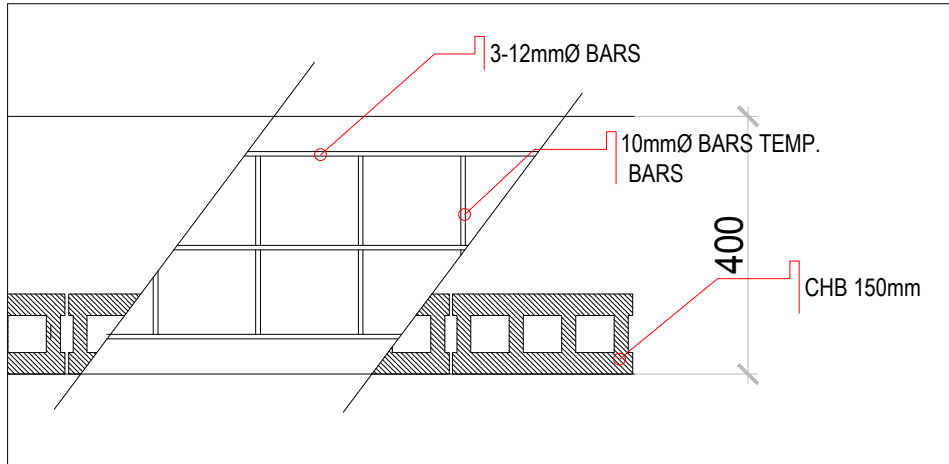
1 S-02 FENCE 1 WALL FOOTING DETAIL 1:50M
