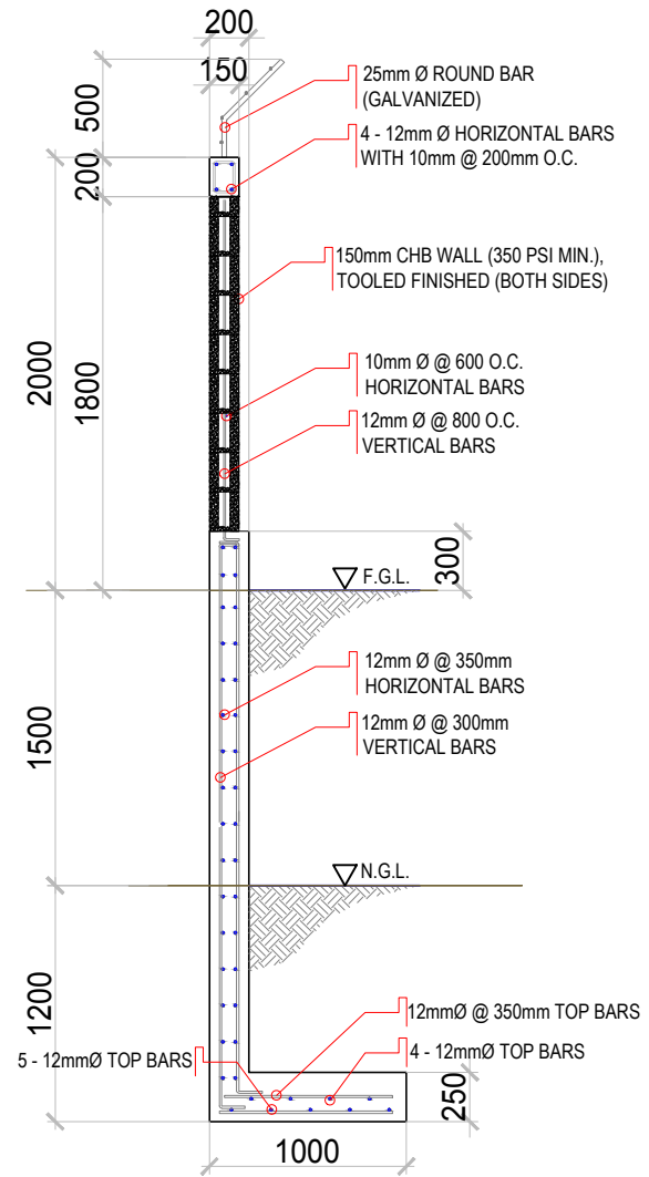
FENCE 2 WALL FOOTING SECTION
