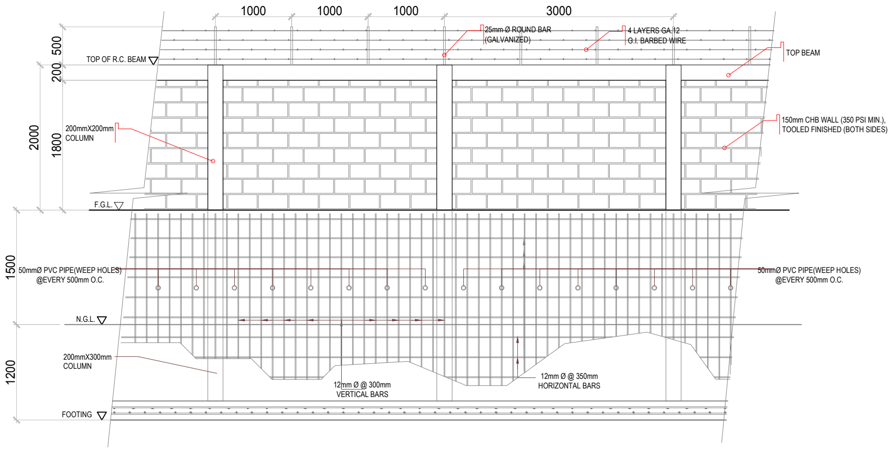
FENCE 2 1 A-03 TYPICAL ELEVATION 1:50M
