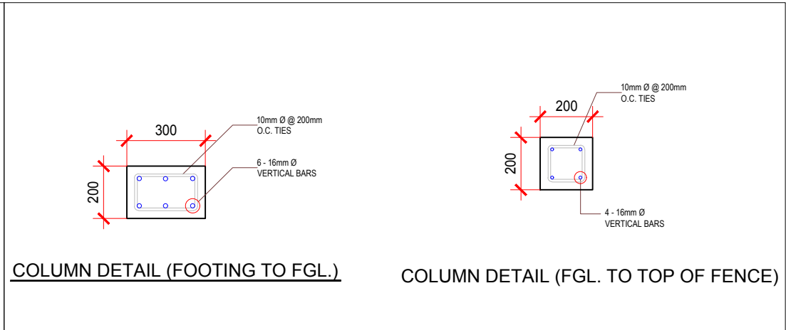
2 S-02 COLUMN DETAIL 1:50M
