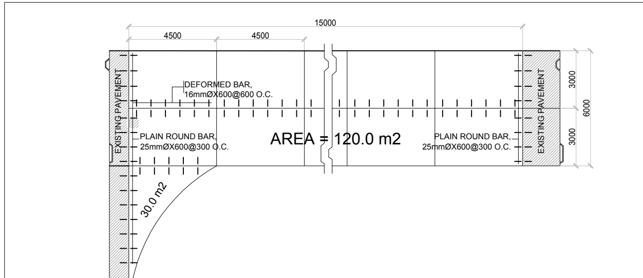
1 ROAD LAYOUT (A=120.0 M 2 ) A-07
