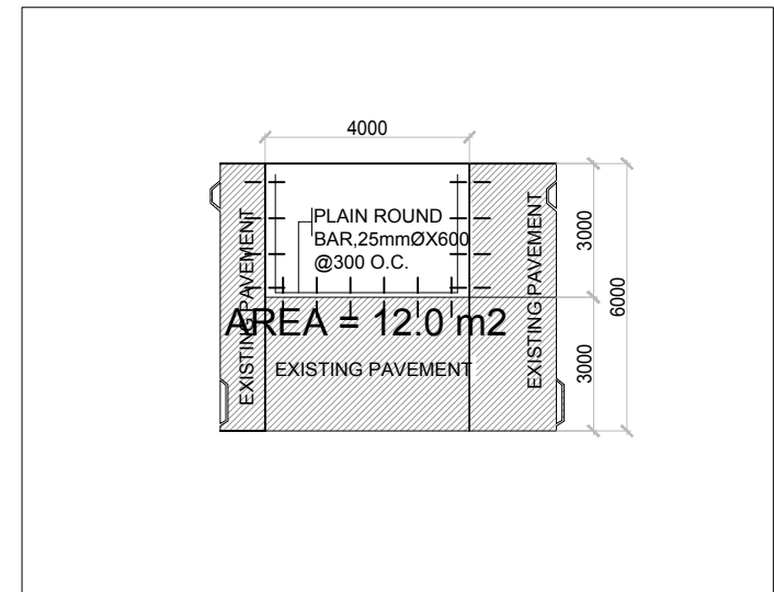
4 ROAD LAYOUT (A=12.0 M2) A-06
