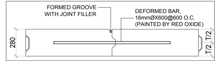
2 SECTION - A (LONGITUDINAL JOINTS) A-02
