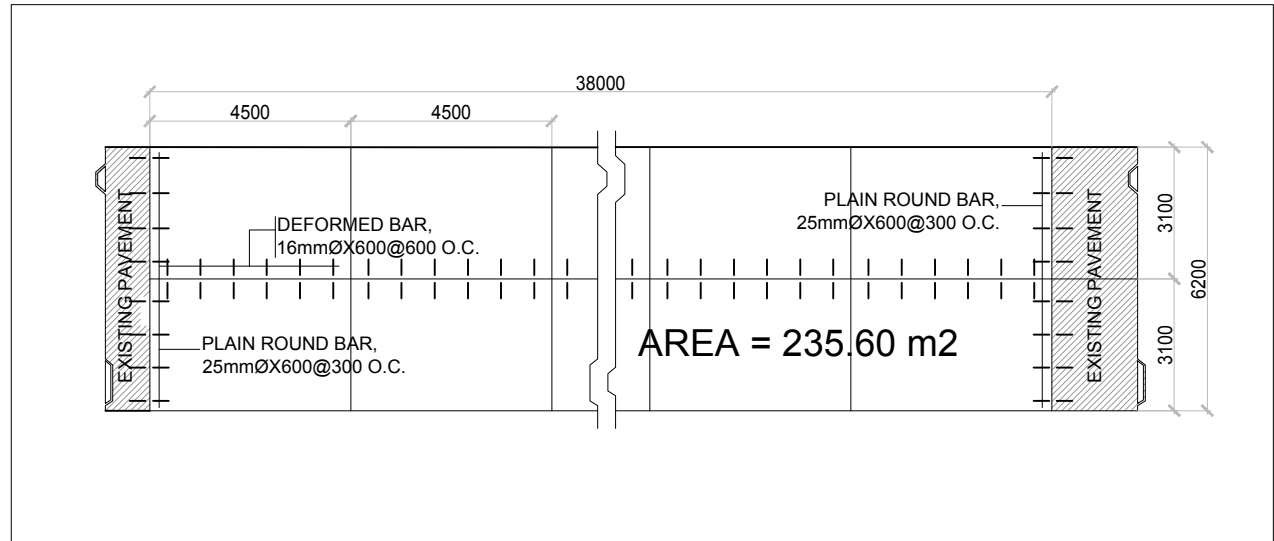
2 ROAD LAYOUT (A=235.60 M2) A-06
