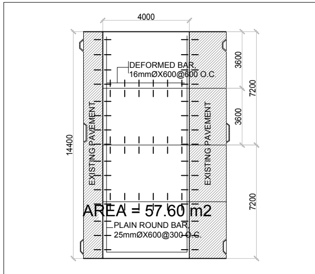
1 ROAD LAYOUT (A=57.60 M2) A-06
