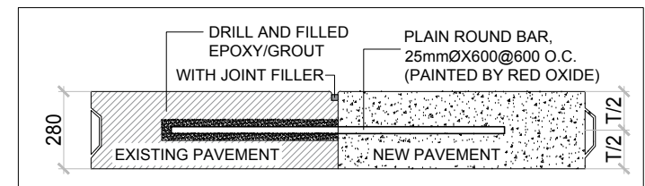
5 SECTION (NEW AND EXISTING PCCP) A-02
