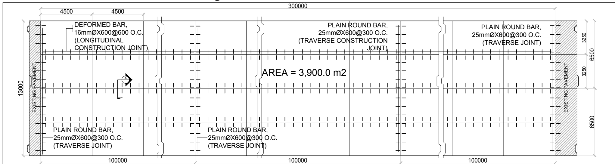
2 ROAD LAYOUT (A=3,900.0 M2) A-04
