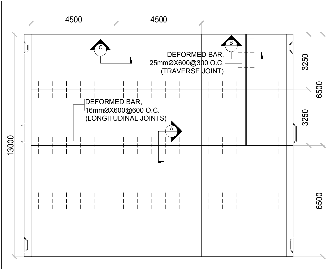
1 TYPICAL PLAN FOR 4 LANE PAVEMENT LAYOUT A-02
