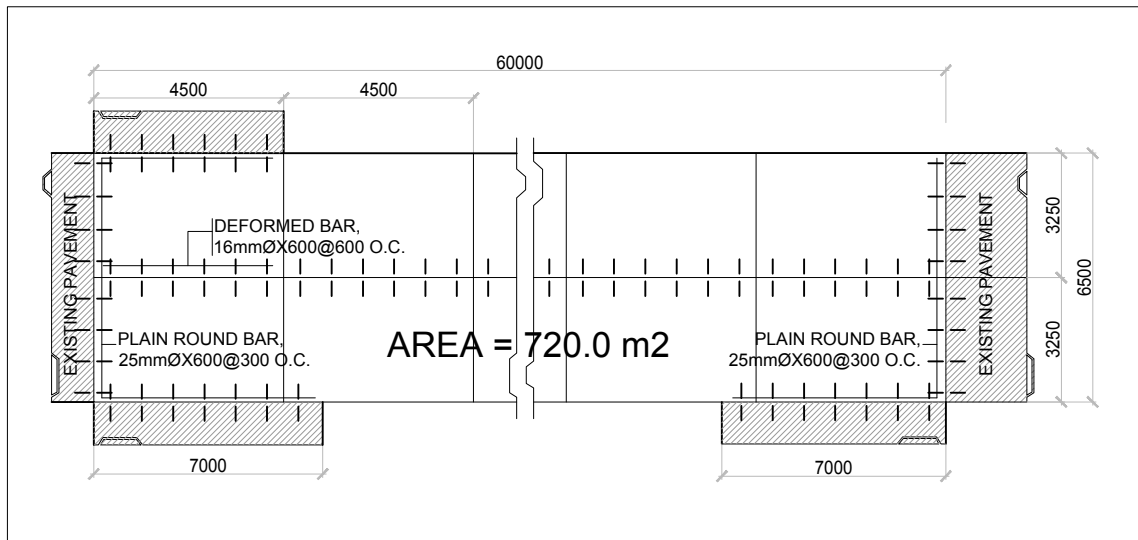
3 ROAD LAYOUT (A=720.0 M2) A-06
