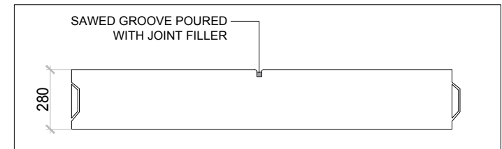
4 SECTION - C (CONTRACTION JOINTS) A-02
