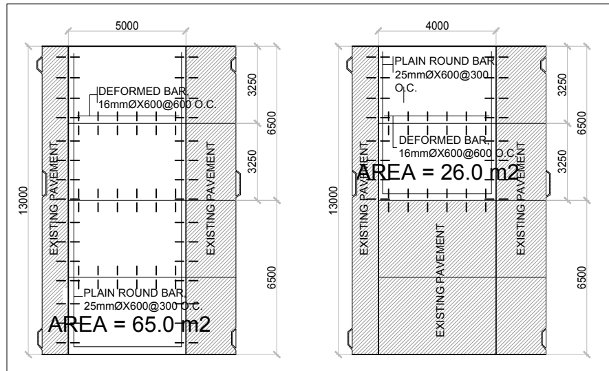
2 ROAD LAYOUT (A=91.0 M 2 ) A-05
