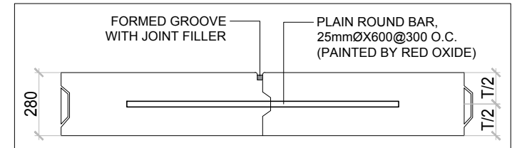
3 SECTION - B (TRAVERSE JOINTS) A-02
