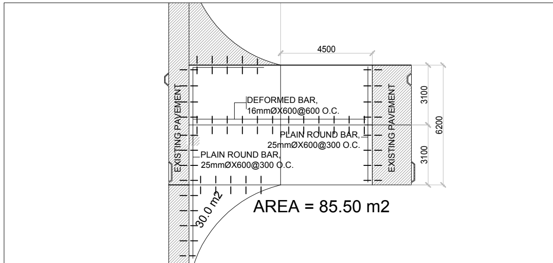
2 ROAD LAYOUT (A=85.50 M 2 ) A-07
