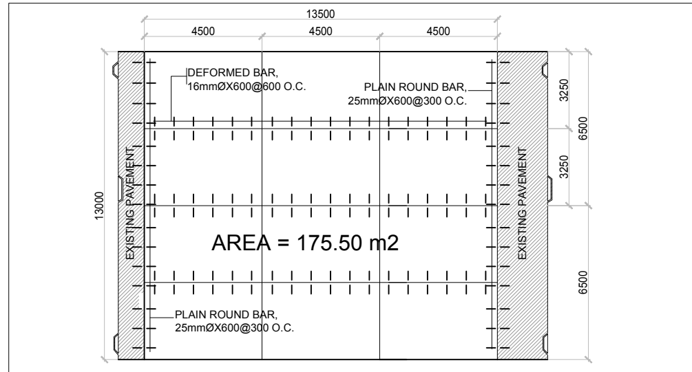
1 ROAD LAYOUT (A=175.50 M 2 ) A-05
