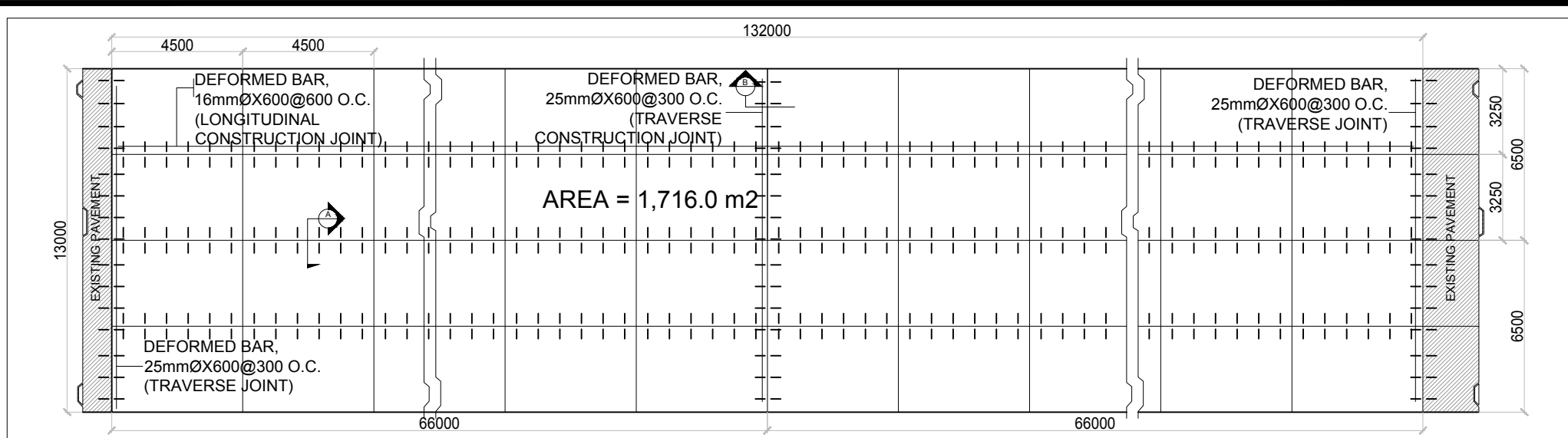
1 ROAD LAYOUT (A=1,716.0 M2) A-04
