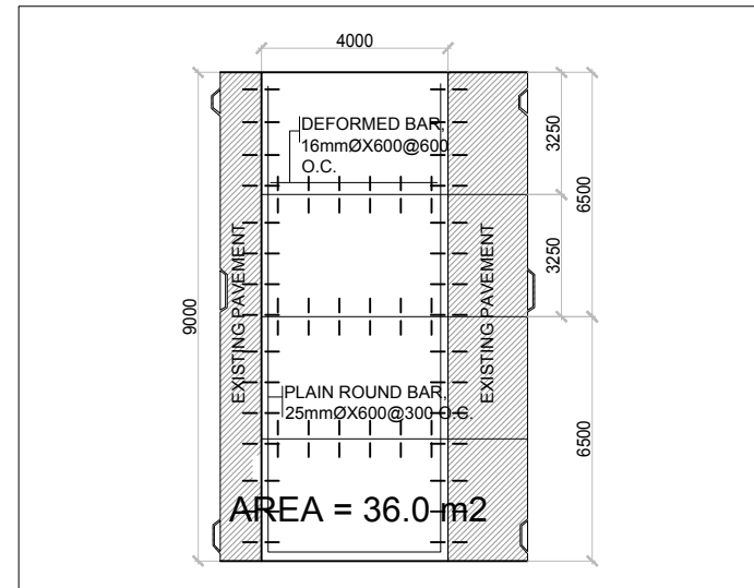
3 ROAD LAYOUT (A=36.0 M 2 ) A-05
