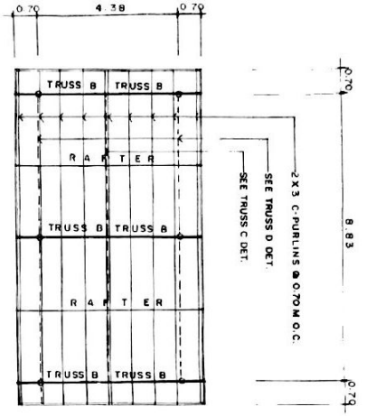
ROOF FRAMING PLAN SCALE: 1/80
