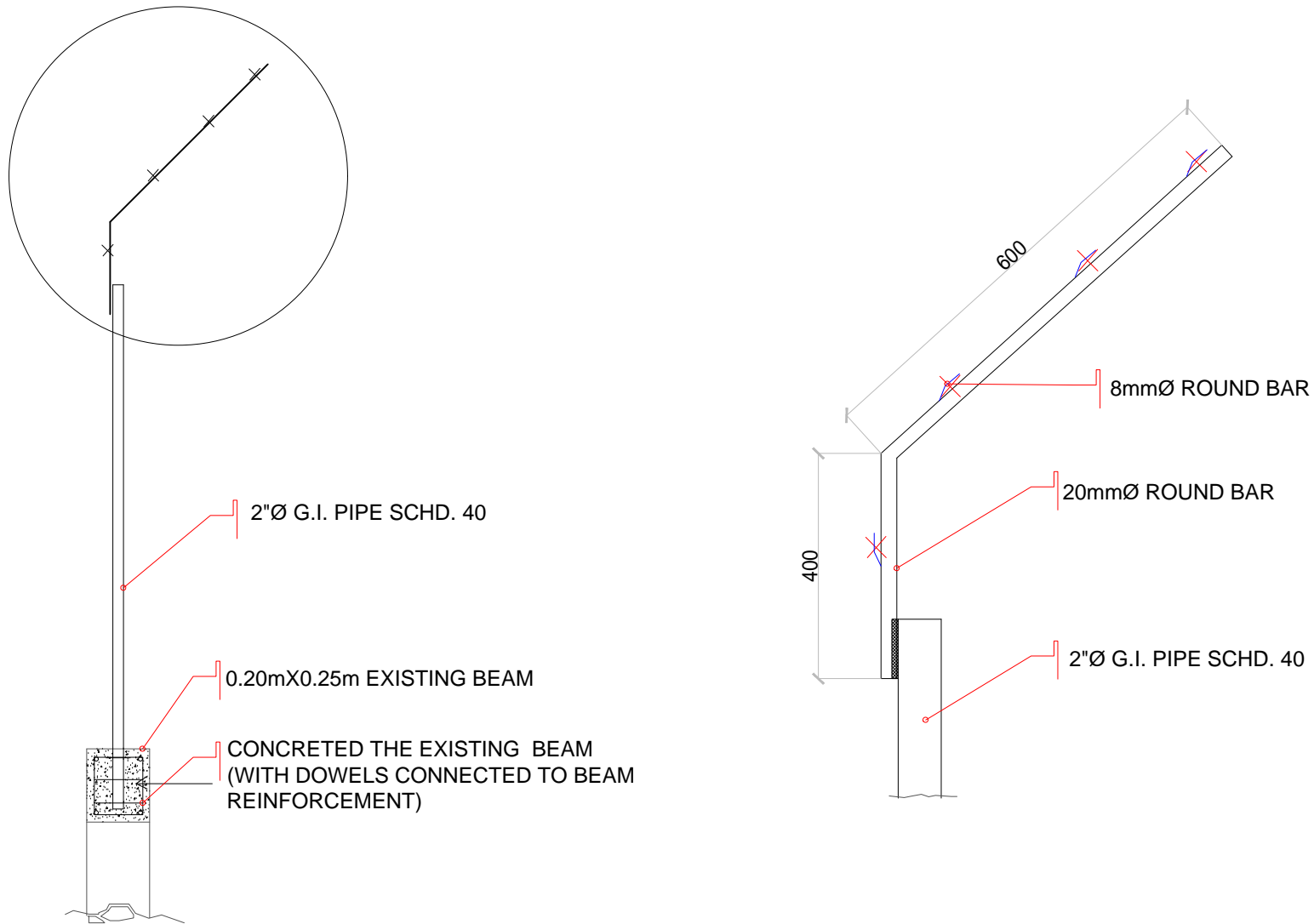
TYPICAL ELEVATION 1:50M
