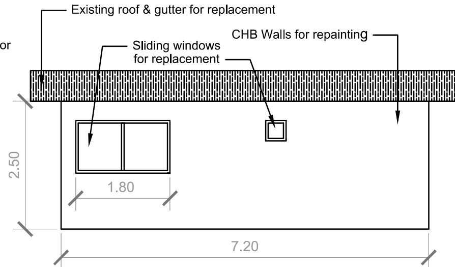
5 RIGHT ELEVATION SCALE
