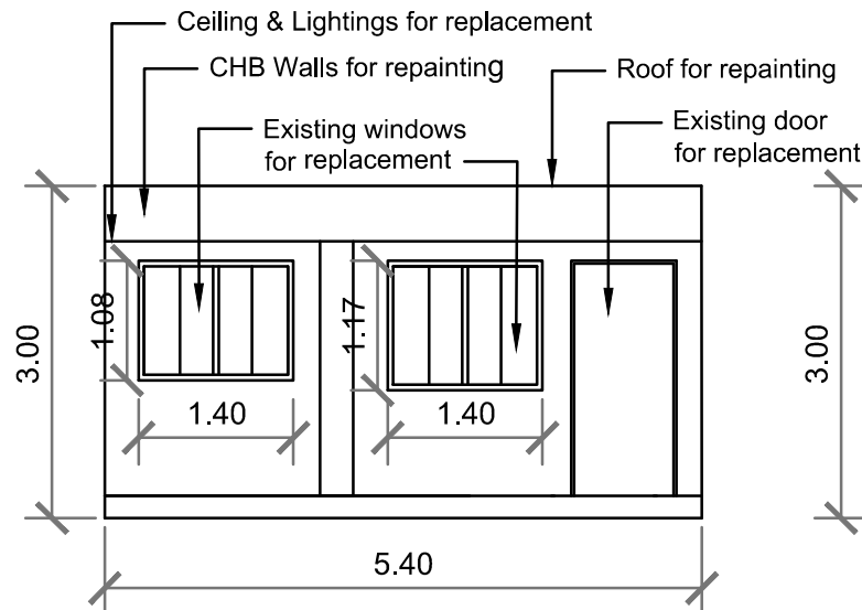
2 FRONT ELEVATION SCALE
