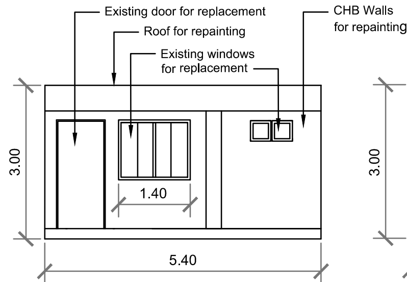
3 REAR ELEVATION SCALE
