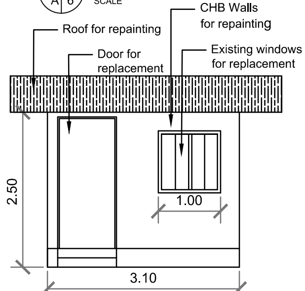
5 A 6 SCALE RIGHT ELEVATION
