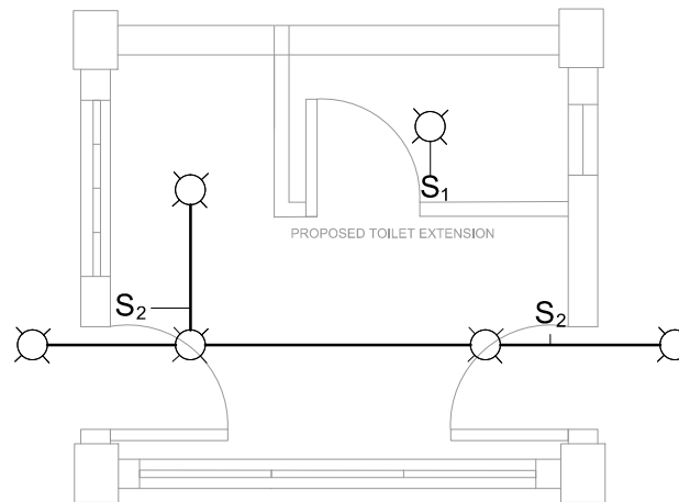
GH-4 LIGHTING LAYOUT 3 E 1 SCALE
