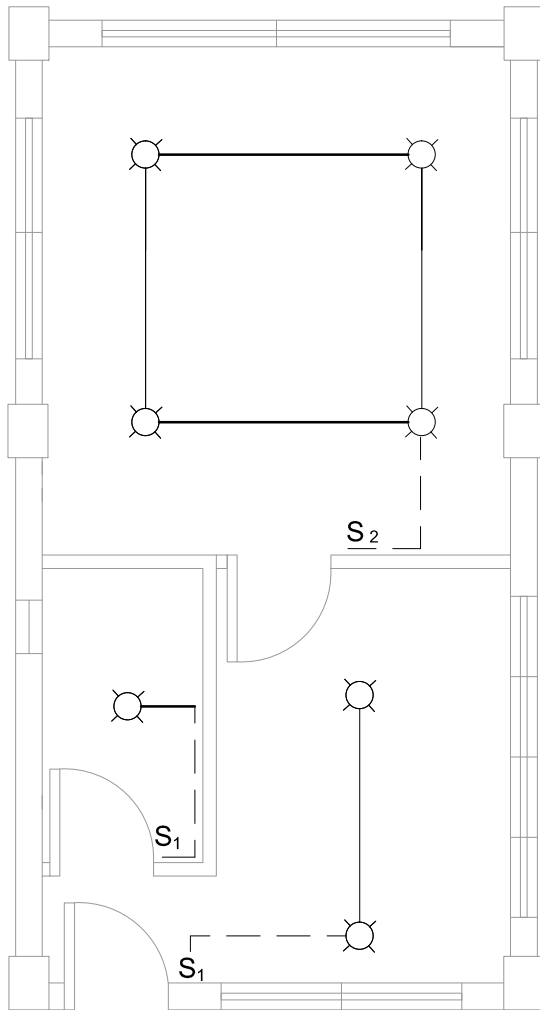
GH-1 LIGHTING LAYOUT 1 E 1 SCALE
