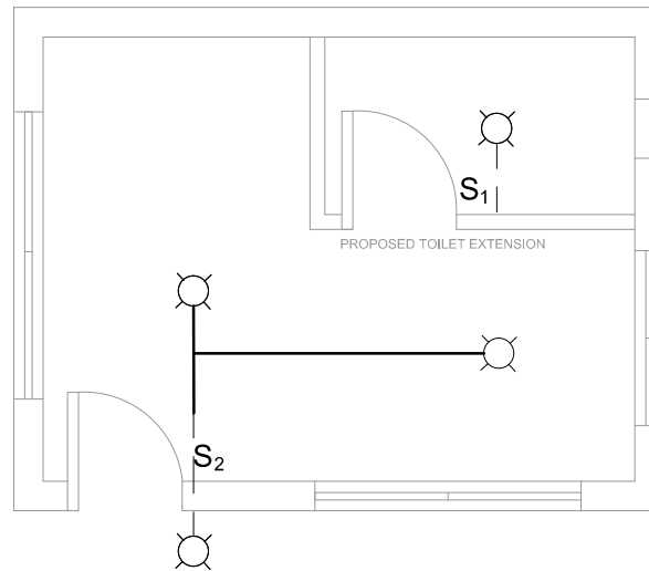
GH-2 LIGHTING LAYOUT 2 E 1 SCALE
