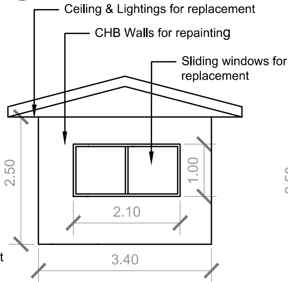
2 FRONT ELEVATION SCALE
