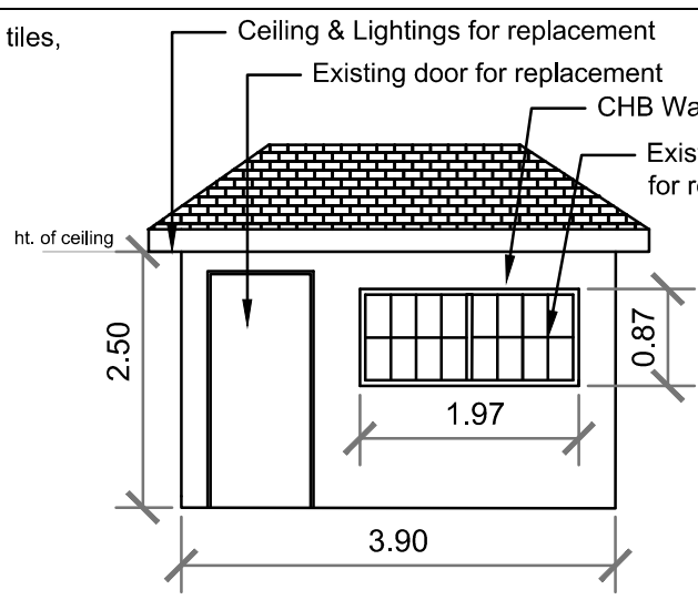
3 FRONT ELEVATION A 3 SCALE
