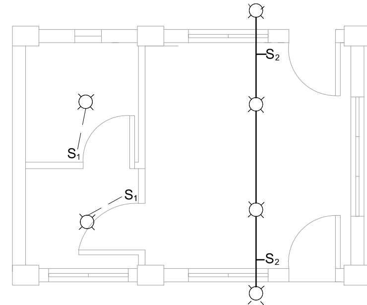
GH-3 LIGHTING LAYOUT 4 E 1 SCALE
