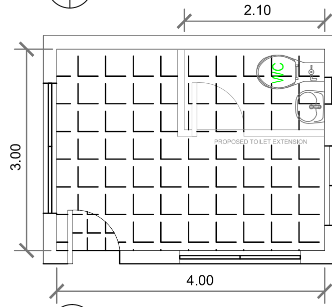
2 PROPOSED FLOOR PLAN A 3 SCALE
