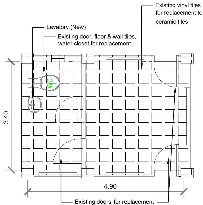
1 EXISTING FLOOR PLAN (GH 3) SCALE
