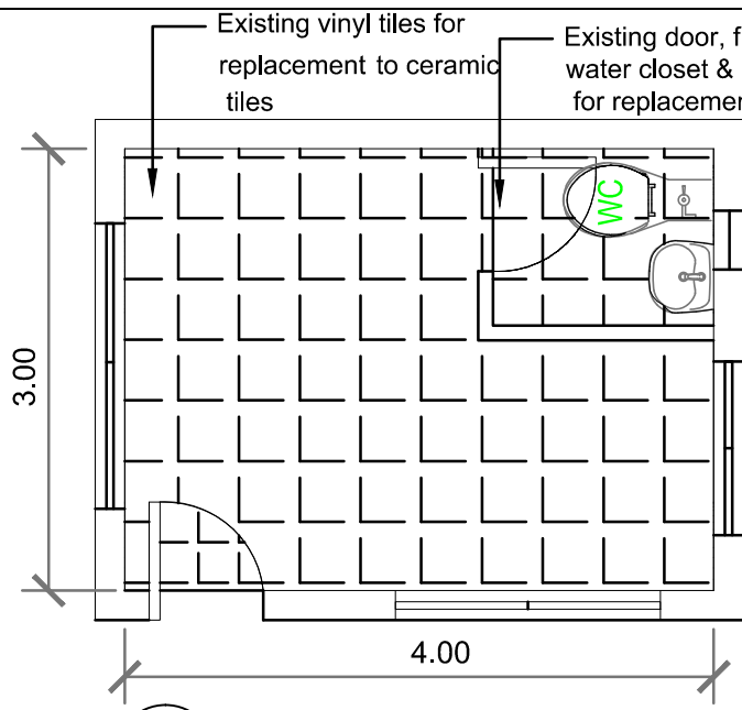
1 EXISTING FLOOR PLAN A 3 SCALE
