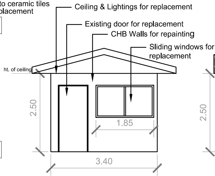
2 FRONT ELEVATION SCALE
