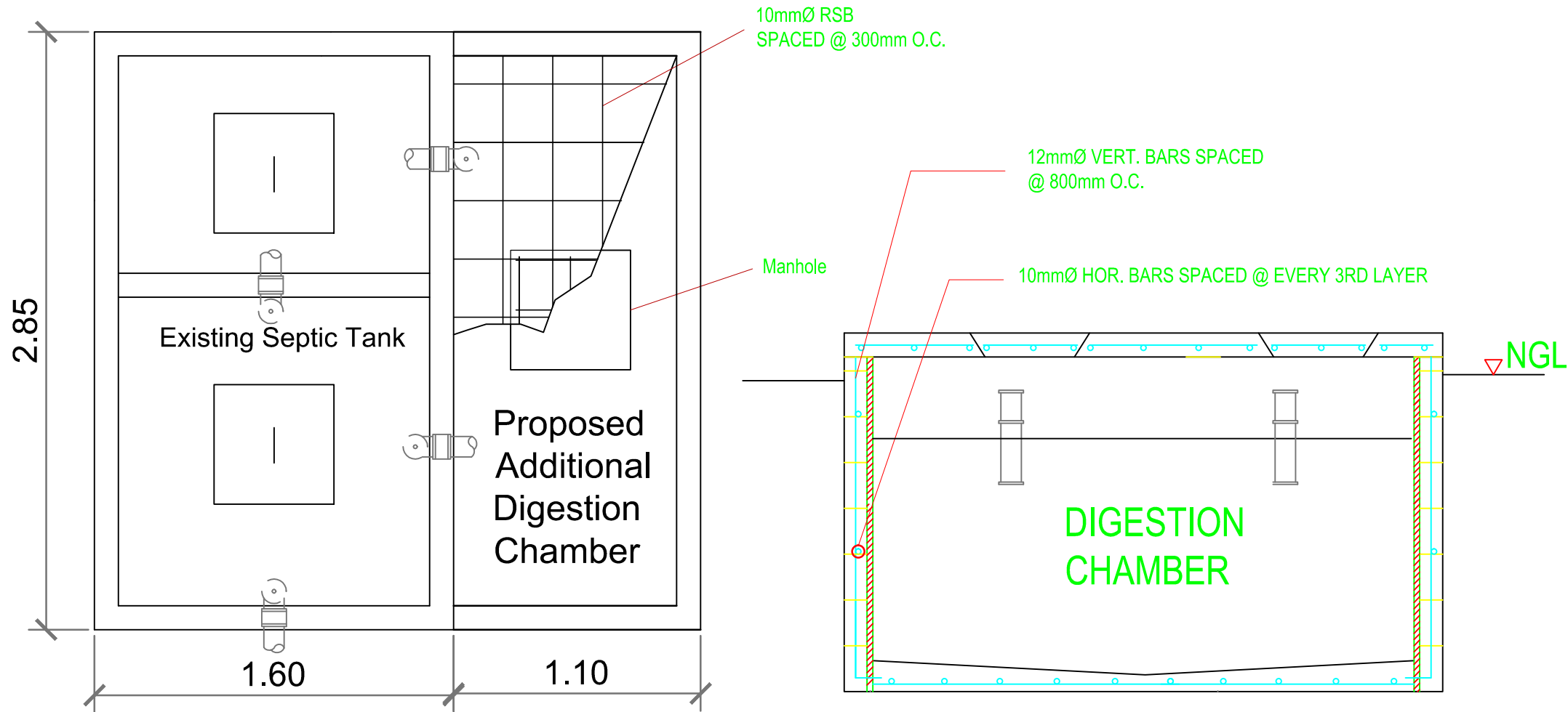
PLAN SEPTIC VAULT 1 P 2 SCALE
