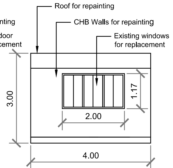
4 RIGHT ELEVATION SCALE
