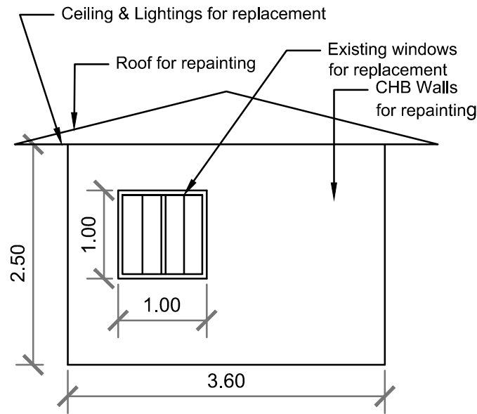
2 A 6 SCALE FRONT ELEVATION
