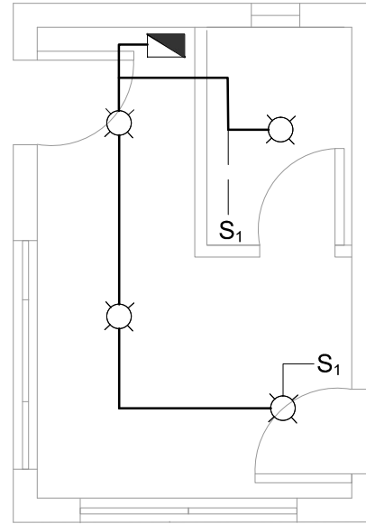
2 GH-6 LIGHTING LAYOUT E 2 SCALE
