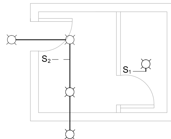
GH-5 LIGHTING LAYOUT 5 E 1 SCALE
