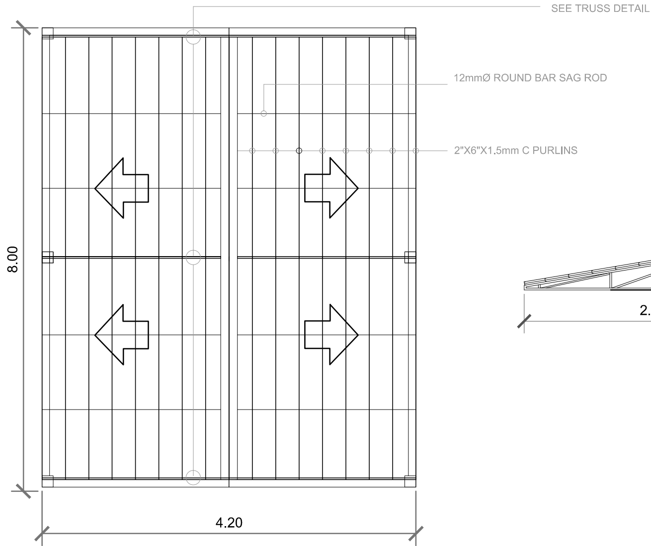
1 S 1 ROOF FRAMING PLAN SCALE
