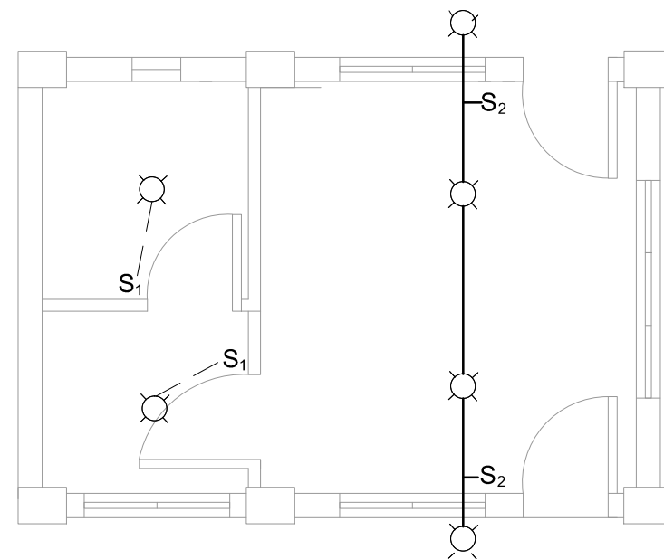
GH-3 LIGHTING LAYOUT 4 E 1 SCALE
